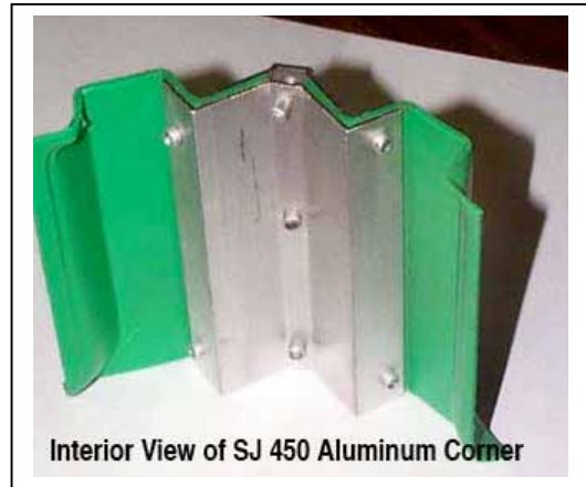
Inside Aluminum Corner for Durability
